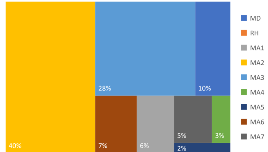
Δ (Mbed)
